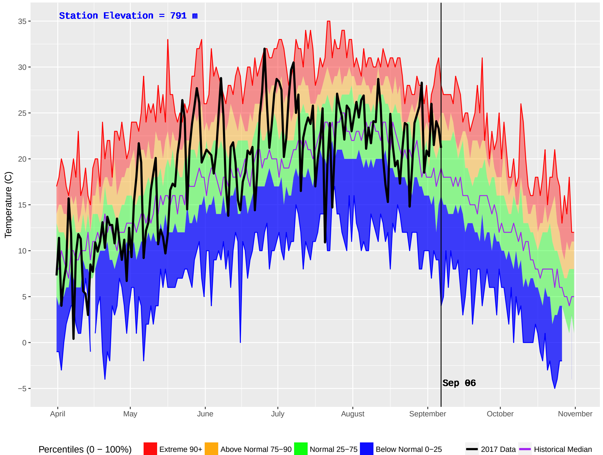
ALEXIS CREEK (209) : Historical (1980–2016) and Current (2017) Noon Temperature
